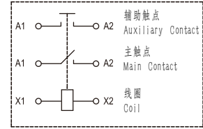
接线图 Coil Wiring Diagram
