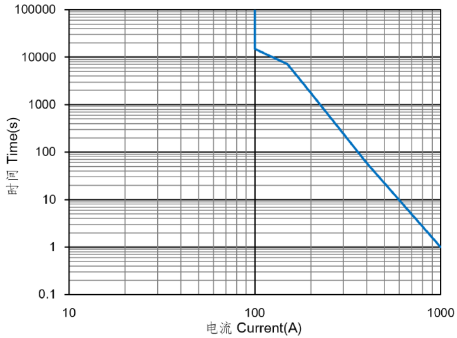
电流承载曲线 Current Carry Curve:
